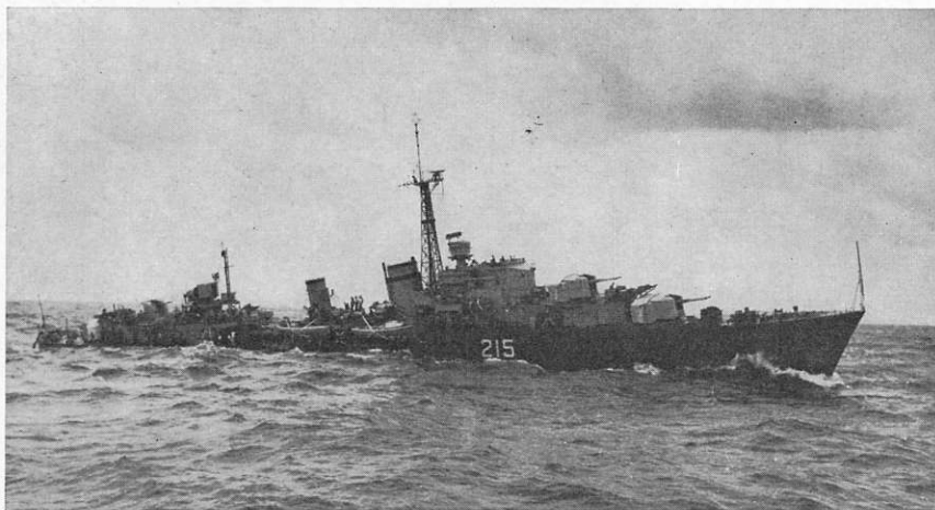
This is the last photograph taken at sea of HMCS "Haida" before the destroyer became jetty-bound as depot ship of the Reserve Fleet in Halifax. It looks as though the "Haida" is down by the stern, but that is only an illusion created by a big roller that has humped up between the camera and the ship and by the fact that the sea has rolled the "Haida" to starboard. ( Mag-1124 ).
