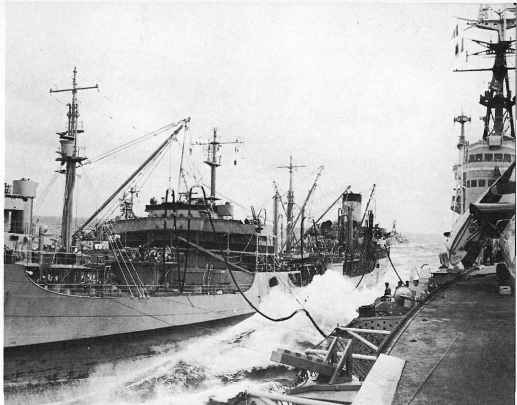
During NATO Exercise New Broom IV, the Magnificent and her destroyer screen rode out a three-day gale in the North Atlantic. The sea was still rough when the exercise ended on September 14, as may be observed from this picture of the "Maggie" oiling on that day from the fleet oiler USS Nantahala . Also visible is the new commodore's bridge, fitted above the compass platform of the carrier's island. (Mag-6584)
