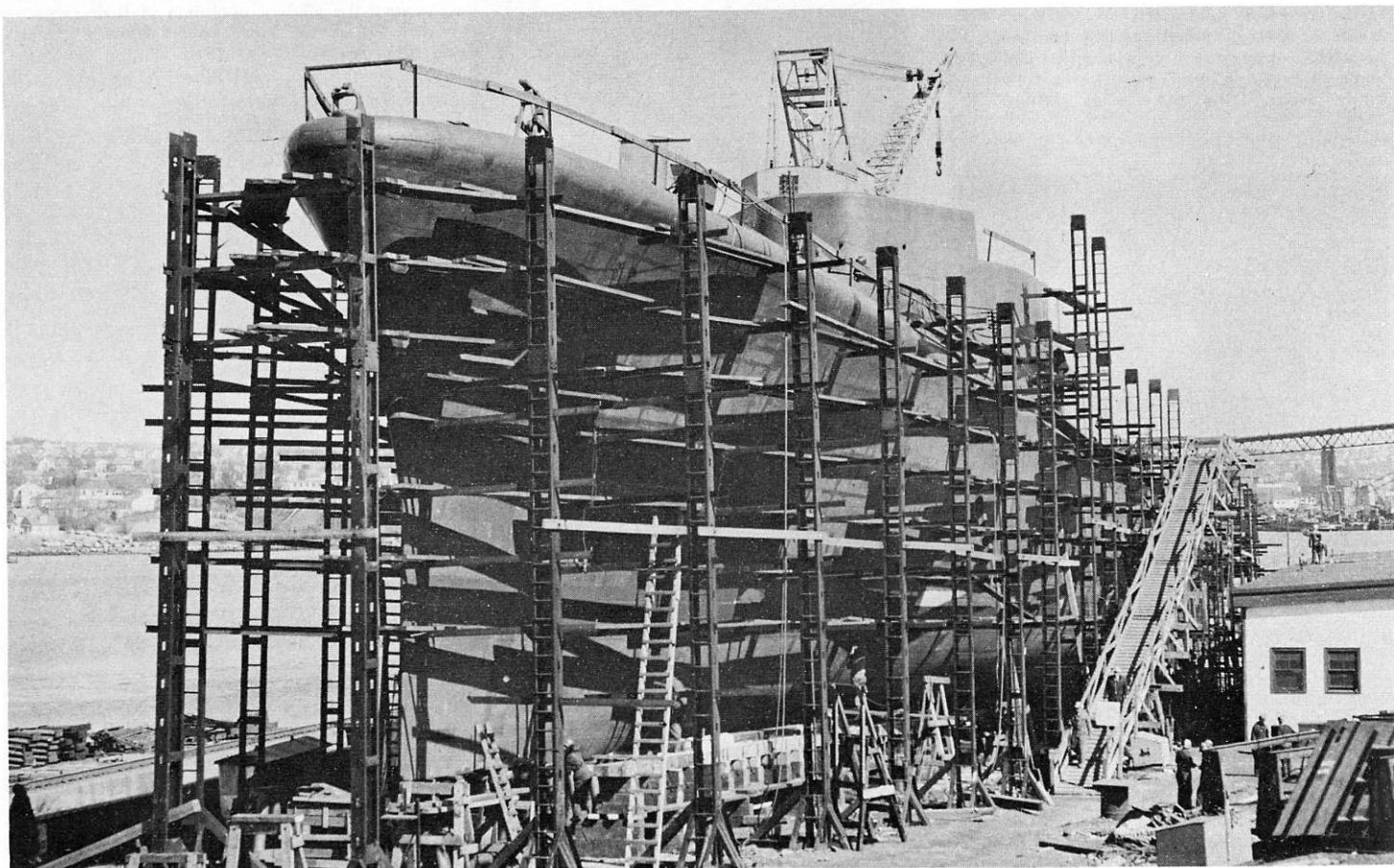
The destroyer escort Annapolis was launched at Dosco Halifax Shipyards April 27. Last to be launched of the six-ship Mackenzie class of Canadian designed and built anti-submarine destroyers, she will be completed in 1964. A helicopter platform and variable depth sonar are included in her construction. (HS-71605)
