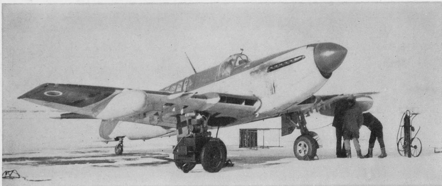
Cold starting tests being carried out on the Firefly 4 at Watson Lake. When the mercury is out of sight, this is not the pleasantest of work.
